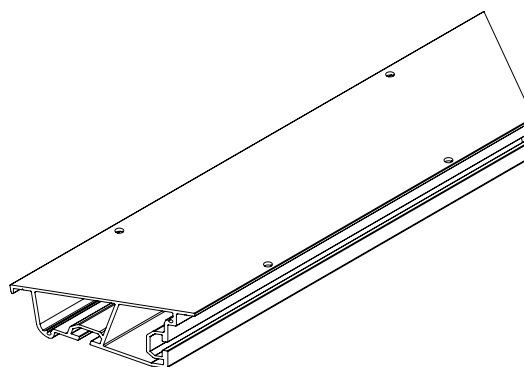
Profile 525 mm
